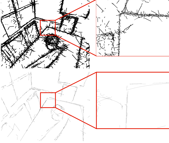
Figure 3. Close up results on the Room2 scene of the Replica dataset. Showing that when trained from COLMAP initialised poses, EdgeGaussians reconstructs the scene as many fragmented line segments. Whereas EdgeSplats, while still having some duplicates produces fewer, cleaner segments
