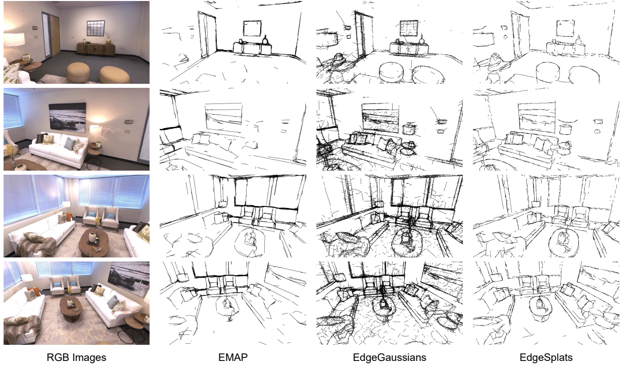
Figure 2. Qualitative results on Room0 of the Replica dataset. Comparing the outputs of EMAP, EdgeGaussians, and EdgeSplats against the input PidiNet edge maps. All methods were initialised with COLMAP estimated poses and seed points. EdgeSplats is less noisy than EdgeGaussians, whilst being more complete than EMAP.
