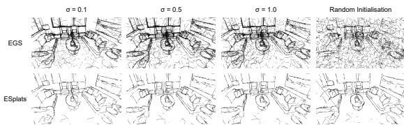
Figure 4. Visualisation of results in Tab.2. We show that the reconstruction provided by EdgeSplats remains consistent with increasing noise level on the initial points.
