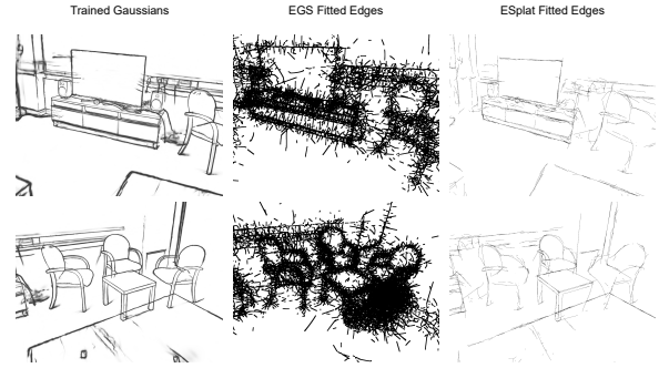
Figure 8. Preliminary results on the Living Lab dataset [17]. A dataset captured on an uncalibrated, handheld device, with estimated points and poses from COLMAP. Highlighting the contrast between EGS and EdgeSplats abilities to adapt to custom data.
