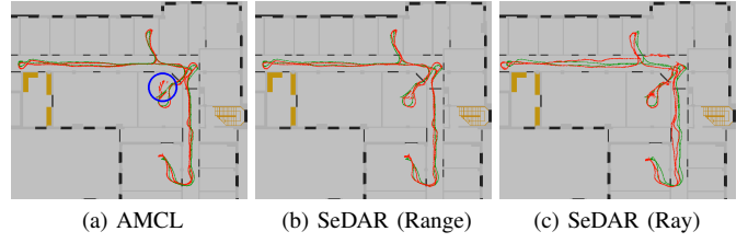
Fig. 5: Estimated path from room-level initialisations.
