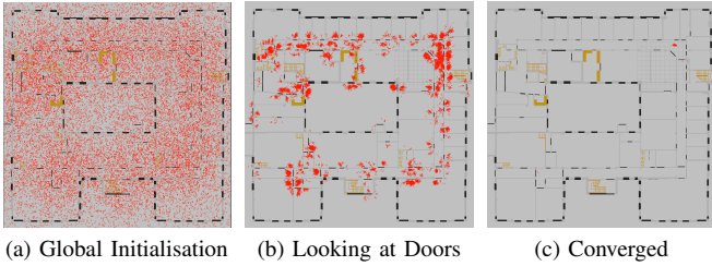
Fig. 6: Qualitative view of Localisation in different modalities.
