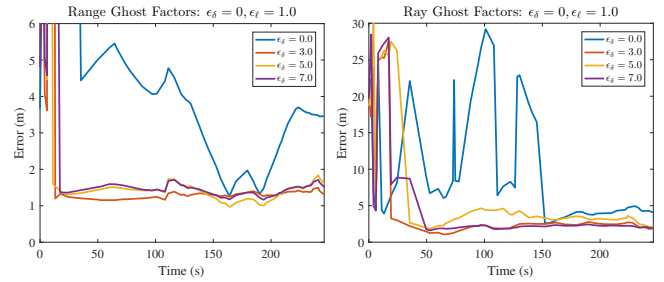
(a) Range-Based (b) Ray-Based
