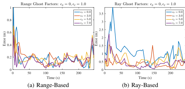
Fig. 9: Different ghost factors ( \epsilon_g ), room-level initialisation. ghost factor of \epsilon_g = 3.0 . In this scenario, inaccuracies in both the map and the sensing modalities allow for otherwise correct particles to be heavily penalised by an aggressive ghost factor. Both of these results are reflected in figures 9a and 9b.
