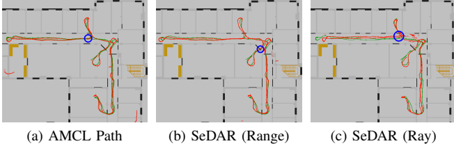
Fig. 7: Estimated path from global initialisations.
