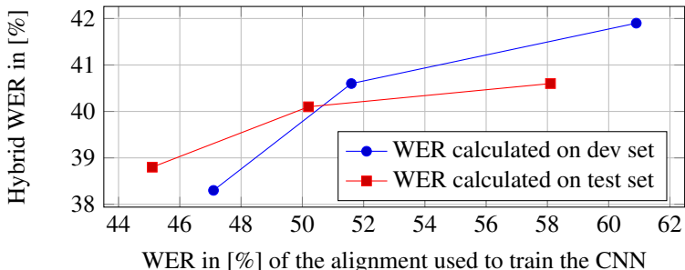
Figure 2: Impact of alignment: continuous sign language recognition results on RWTH-PHOENIX-Weather 2014 Multisigner showing how the initial alignment impacts the CNN learning and subsequent hybrid modelling.
