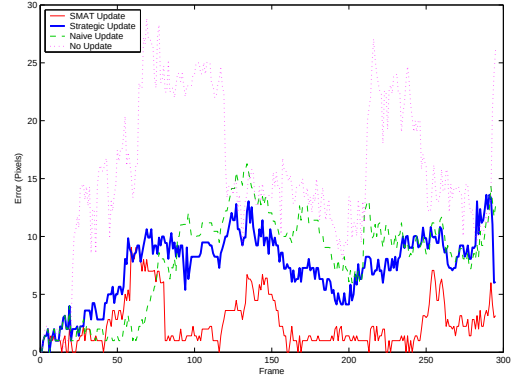
Figure 4. Error plot for “Sign” sequence
