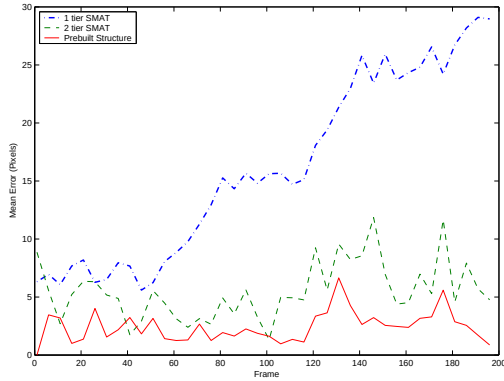
Figure 6. Error plot for “Rhino” sequence
