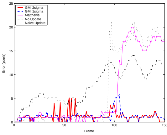
Figure 2. Error Rates for Different Tracking Algorithms
