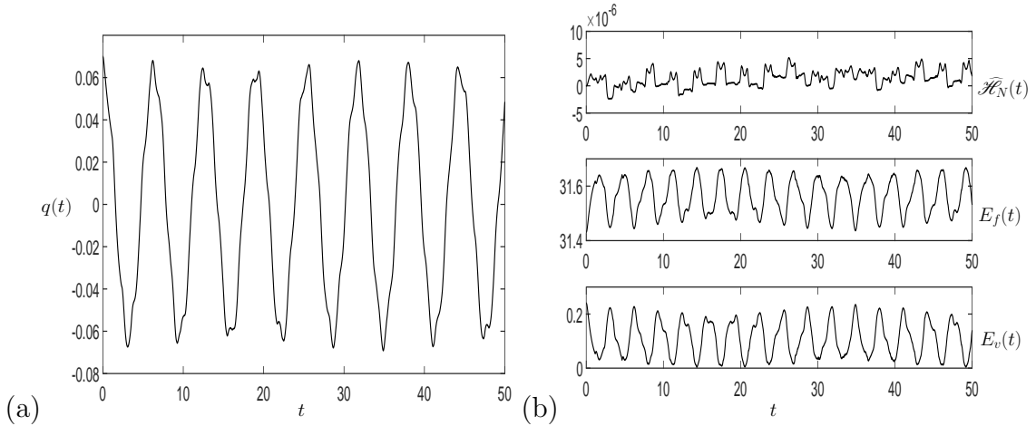
Figure 8: (a) The vessel displacement q(t) and (b) E_f(t) , E_v(t) and \widehat{\mathcal{H}}_N(t) for the initial condition \widehat{q}_1 = \widehat{q}_2 = 0 , \widehat{q} \neq 0 and the initial parameter values given by column 4 of Table 1.
