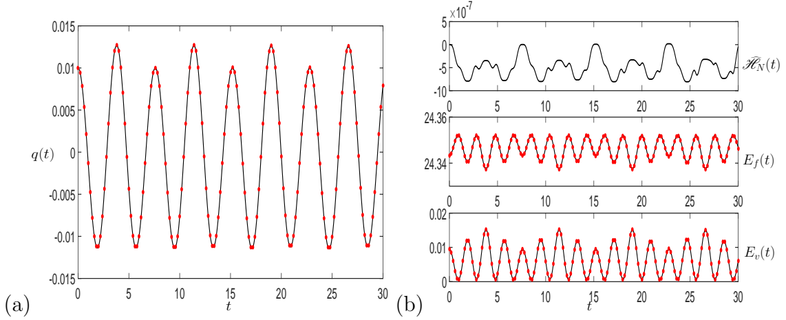
Figure 6: (a) The vessel displacement q(t) and (b) E_f(t) , E_v(t) and \widehat{\mathcal{H}}_N(t) for the initial condition \widehat{q}_1 = 0 , \widehat{q}_2 \neq \widehat{q} and the initial parameter values given in column 4 of Table 1. The dots in panel (a) represent the f-wave solution from [1].
