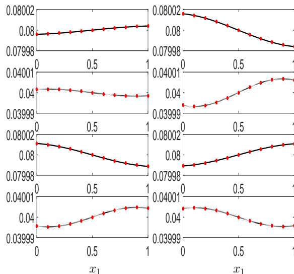
Figure 14: The interface positions h_1(x_1, t) (solid line, upper panels) and h_1(x_1, t) + h_2(x_1, t) (dotted line, lower panels) for the results in figure 4 at, top 2 rows: t = 10 and t = 20 , bottom 2 rows: t = 30 and t = 40 . The dots represent the exact linear solution (C-86) for the lowest frequency mode. The rigid lid is at h_1^0 + h_2^0 + h_3^0 = 0.12 m.
