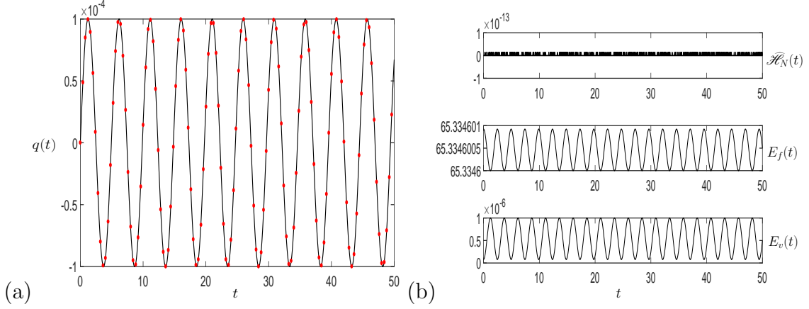
Figure 2: (a) The vessel displacement q(t) and (b) E_f(t) , E_v(t) and \widehat{\mathcal{H}}_N(t) for the linear initial condition \widehat{q}_1 = \widehat{q}_2 = \widehat{q} and the initial parameter values given in column 1 of Table 1. The dots in panel (a) represent the linear solution (2.33). The value of \omega = 0.8995 .
