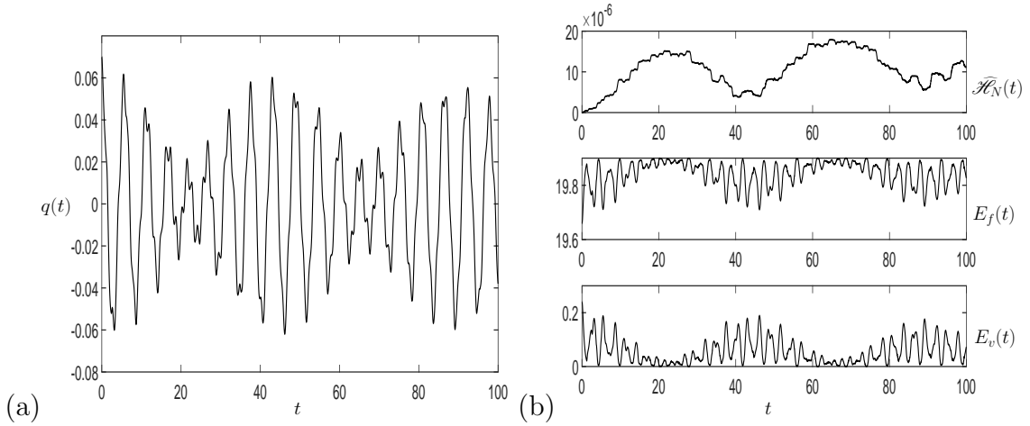
Figure 11: (a) The vessel displacement q(t) and (b) E_f(t) , E_v(t) and \widehat{\mathcal{H}}_N(t) for the initial condition (4.57) and the initial parameter values given in column 5 of Table 1.
