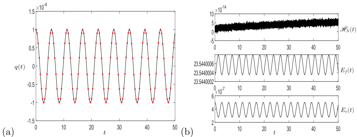
Figure 13: (a) The vessel displacement q(t) and (b) E_f(t) , E_v(t) and \widehat{\mathcal{H}}_N(t) for the linear initial condition Q_1 = 1 and the initial parameter values given in column 1 of table 2. The dots represent the linear solution (C-86) for the lowest frequency mode.
