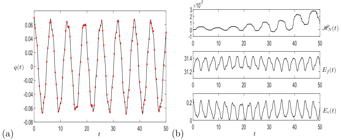
Figure 15: (a) The vessel displacement q(t) and (b) E_f(t) , E_v(t) and \widehat{\mathcal{H}}(t) for the nonlinear initial condition Q_1 = 0 and the initial parameter values given in column 2 of table 2. The dots in represent the two-layer result given by figure 8.
