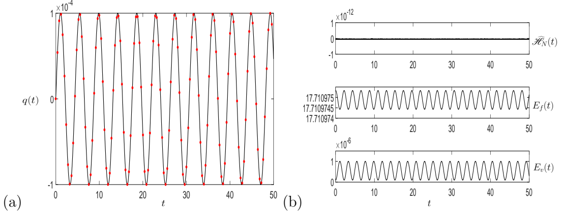
Figure 4: (a) The vessel displacement q(t) and (b) E_f(t) , E_v(t) and \widehat{\mathcal{H}}_N(t) for the linear initial condition \widehat{q}_1 = \widehat{q}_2 = \widehat{q} and the initial parameter values given in column 2 of Table 1. The dots in panel (a) represent the linear solution (2.33). The value of \omega = 1.0980 .
