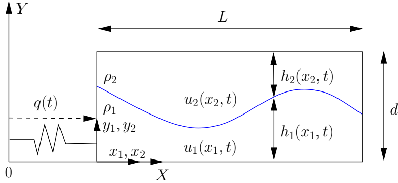
Figure 1: Schematic of the sloshing problem considered for the case of two-fluid layers. Here the vessel is constrained to move in the horizontal direction with displacement q(t) . Here the displacement is determined by attaching the vessel to a nonlinear spring.
