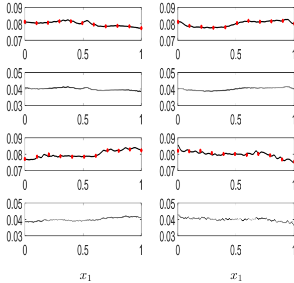
Figure 16: The interface positions h_1(x_1, t) (solid line, upper panels) and h_1(x_1, t) + h_2(x_1, t) (dotted line, lower panels) for the results in figure 8 at, top 2 rows: t = 4 and t = 8 , bottom 2 rows: t = 18 and t = 29 . The dots in the upper panels represent the two-layer result given by figure 9. The rigid lid is at h_1^0 + h_2^0 + h_3^0 = 0.12 m.
