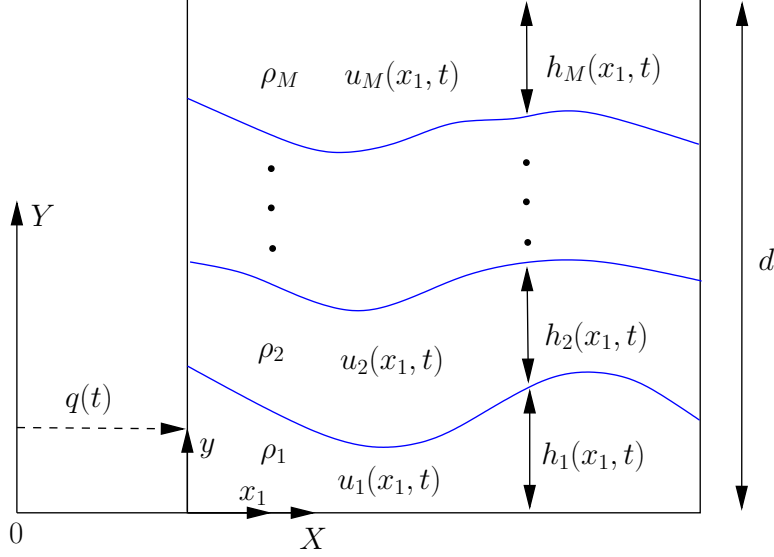
Figure 10: Schematic of M -layer shallow-water sloshing in a moving rectangular vessel, with the constraint x_1 = x_2 = \dots = x_M imposed.
