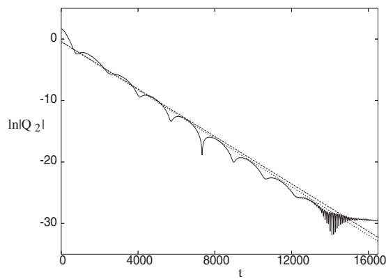
FIG. 11. Plot of \ln|Q_2| against time for the case \delta=1 , \epsilon=0.5 , and r_c=5.2 . The dashed line is the growth rate given by the linear code and the dotted line is the growth rate given by the dominant Landau pole.
